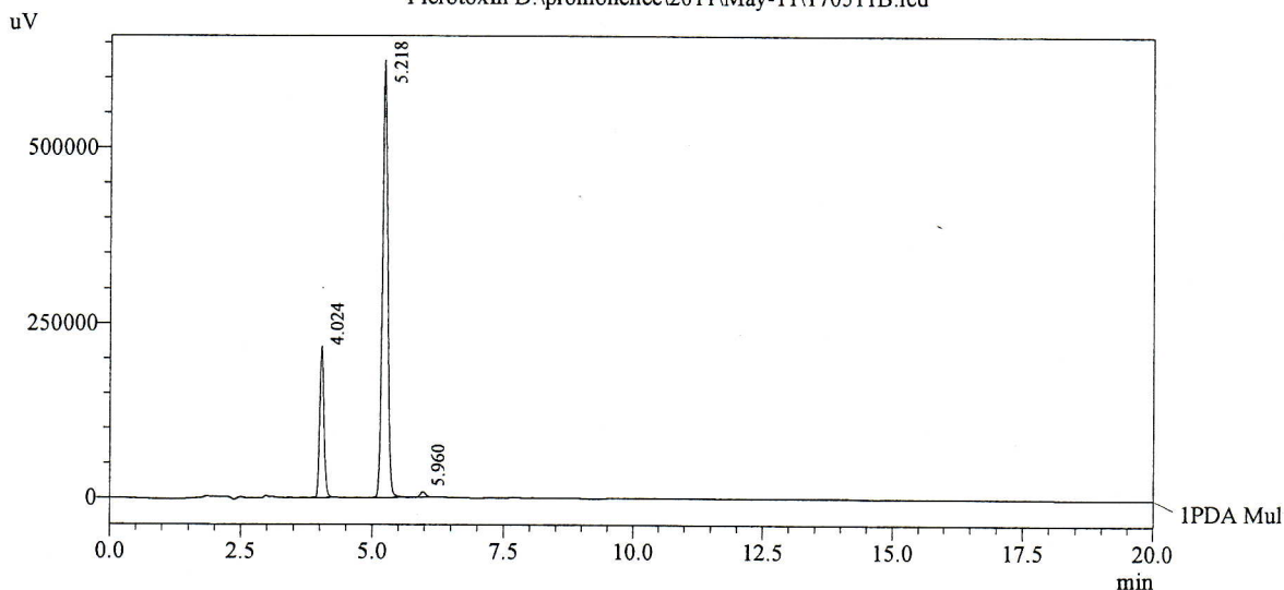
Chromatogram
