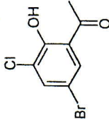
5'-Bromo-3'-chloro-2'-hydroxy acetophenone
