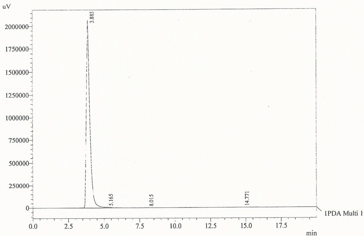
Chromatogram
