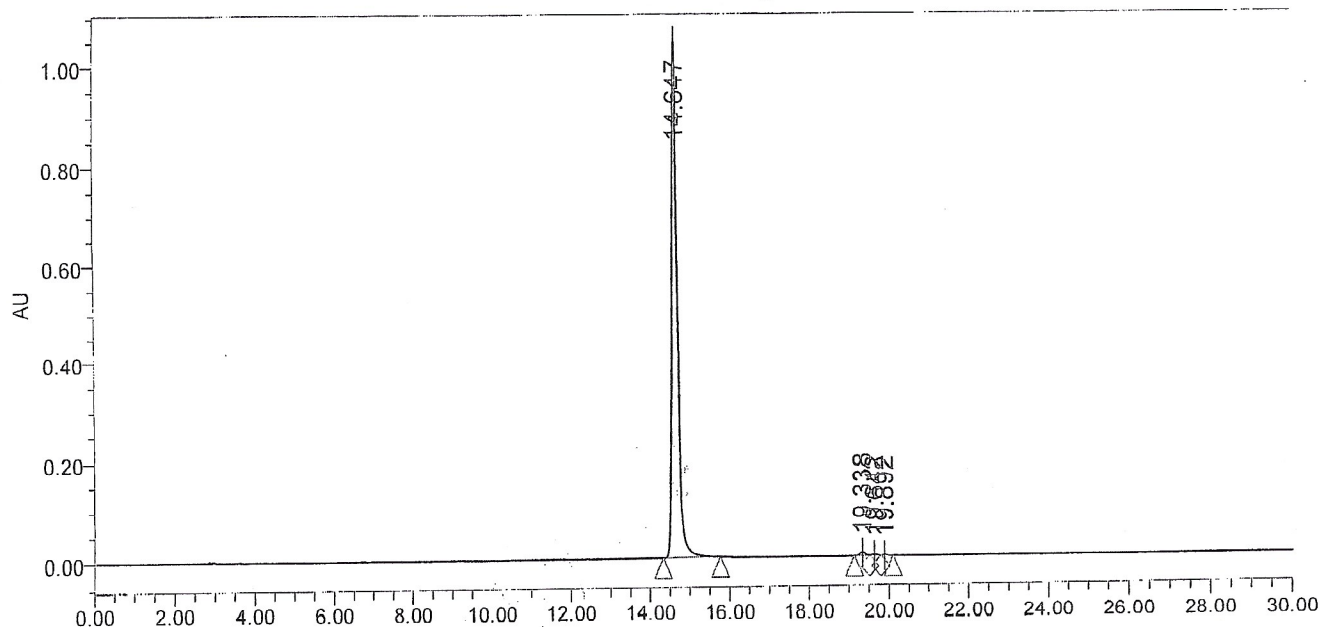
Auto-Scaled Chromatogram
