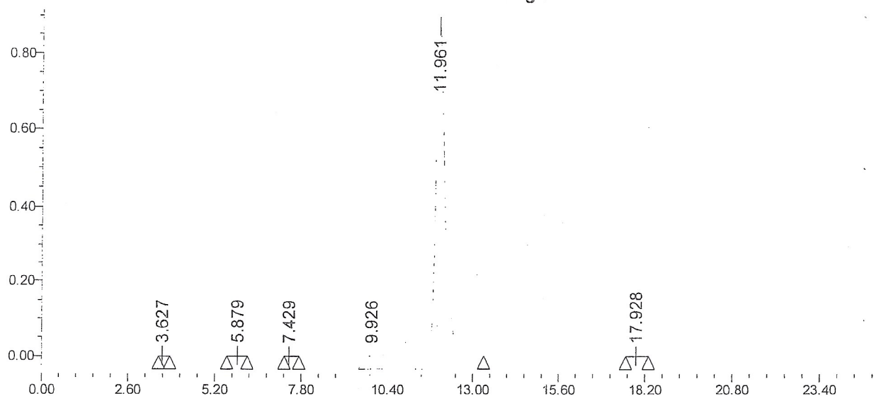
Auto-Scaled Chromatogram
