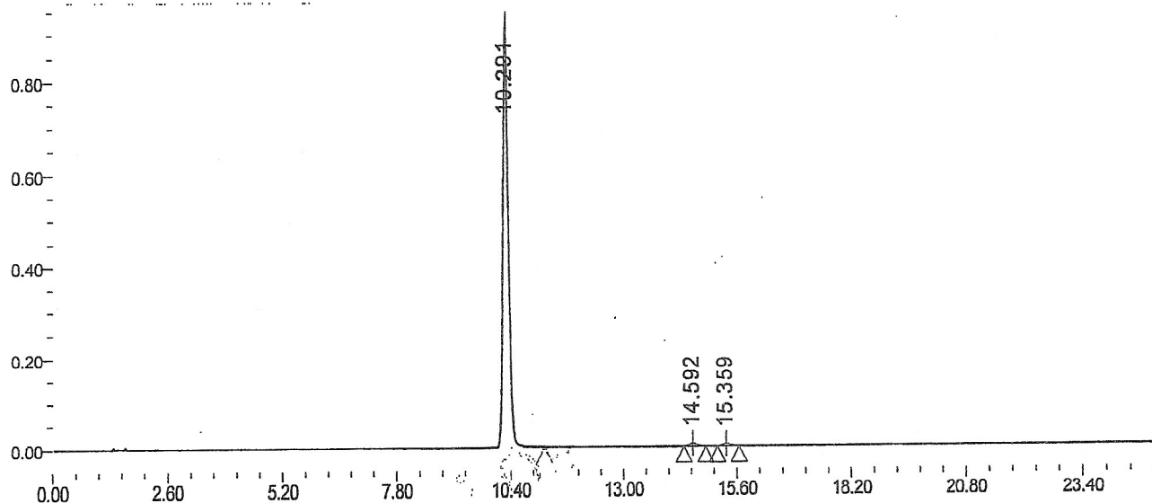
Auto-Scaled Chromatogram
