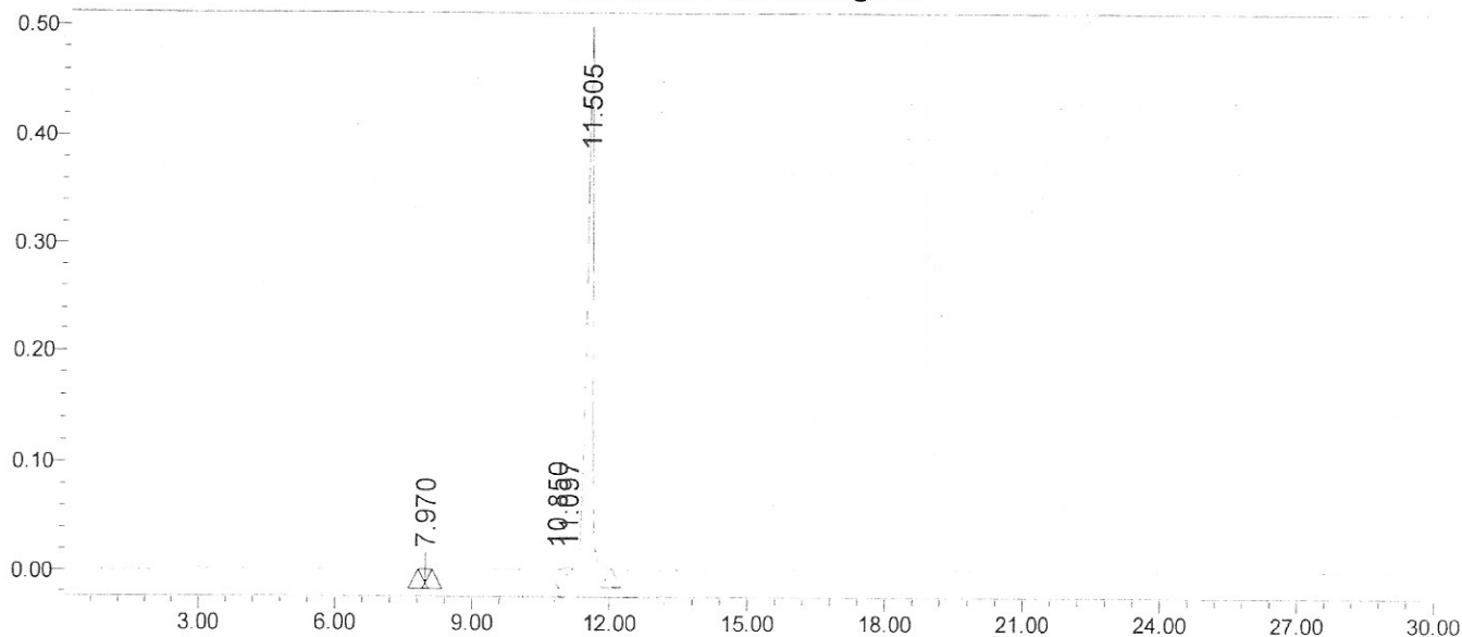
Auto-Scaled Chromatogram
