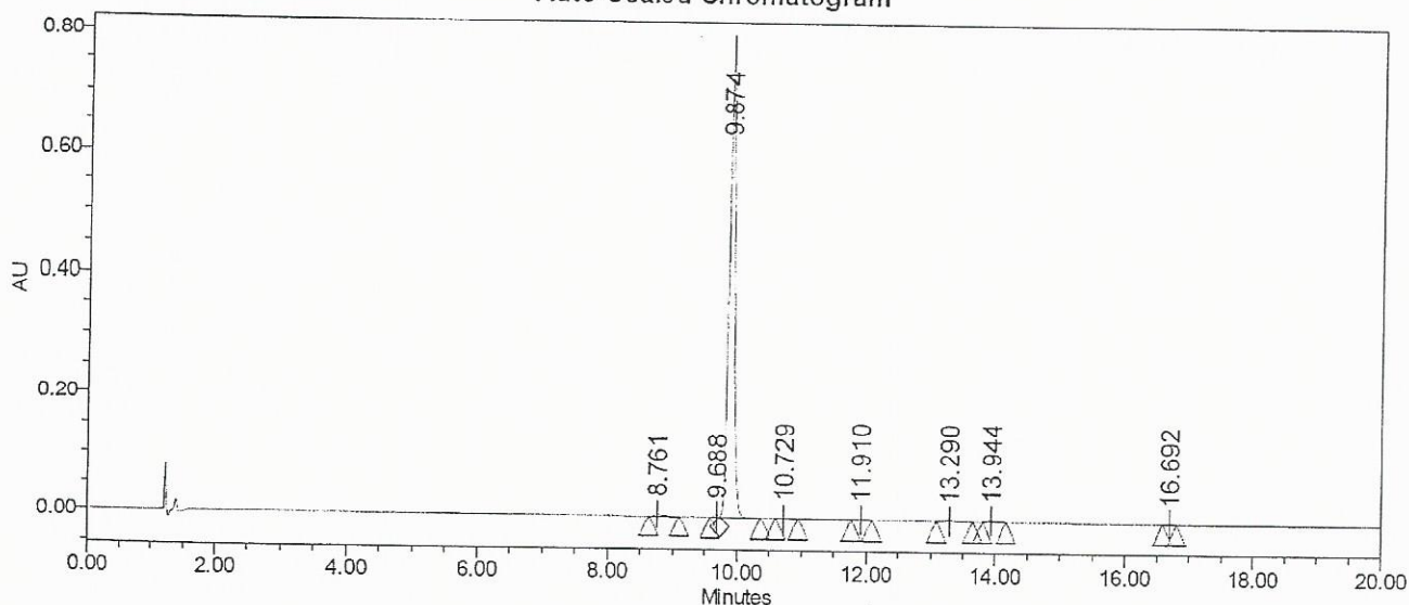
Auto-Scaled Chromatogram
