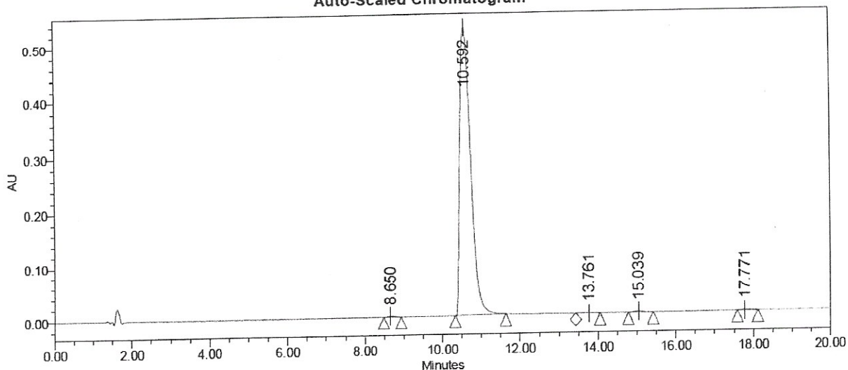
Auto-Scaled Chromatogram
