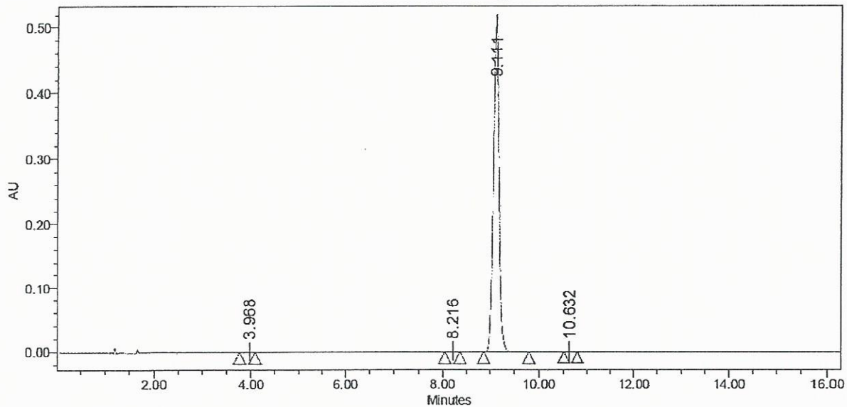
Auto-Scaled Chromatogram
