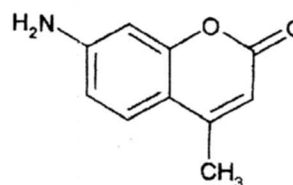
7-Amino-4-methyl coumarin
