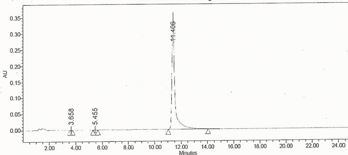
Auto-Scaled Chromatogram
