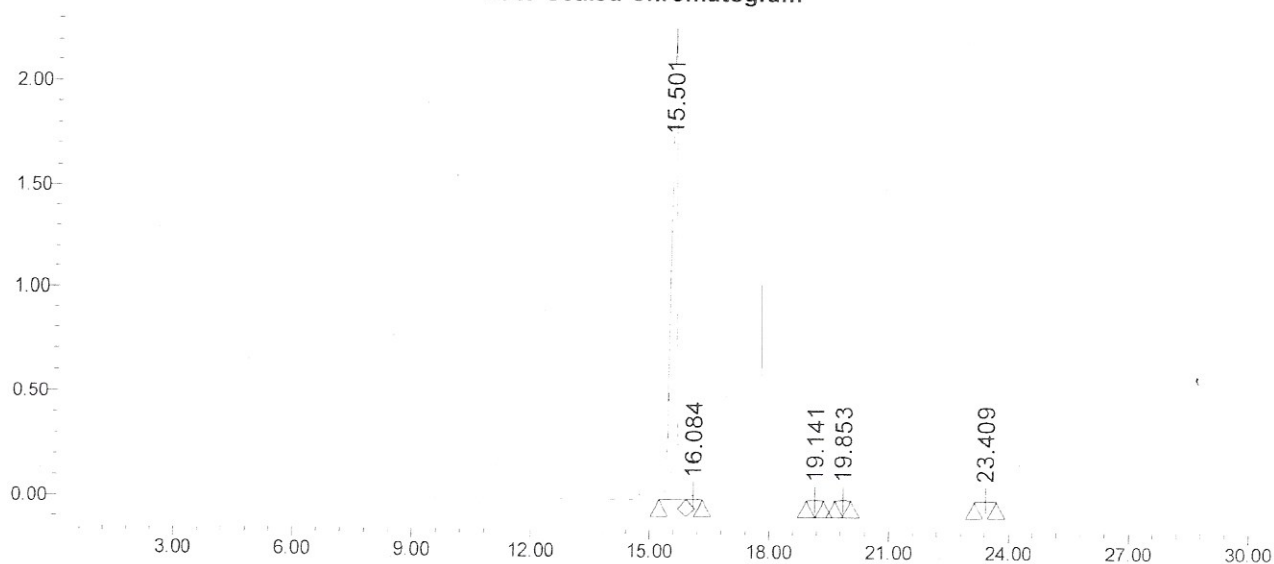
Auto-Scaled Chromatogram
