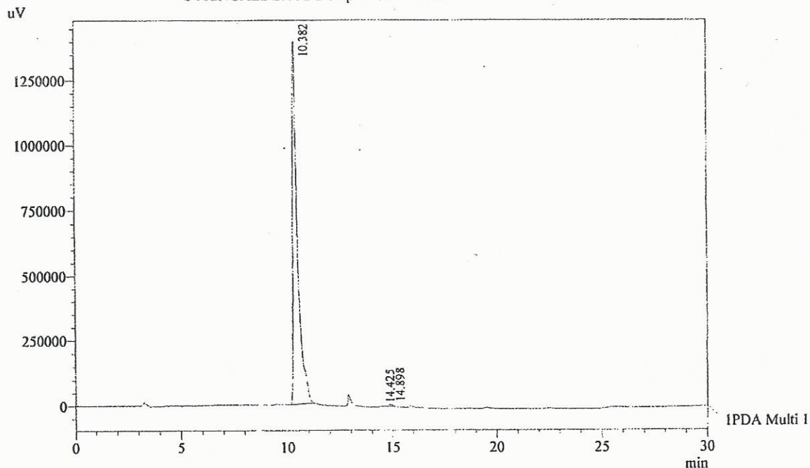
Chromatogram SYRINGALDEHYDE D:\promonence\Data
