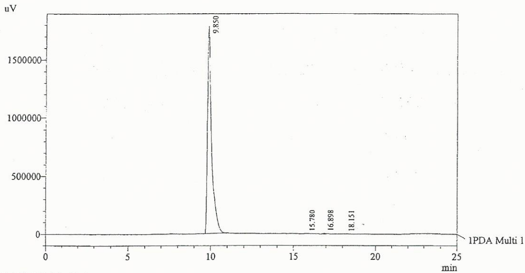
Chromatogram
