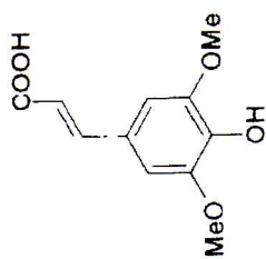
3,5-Dimethoxy-4-hydroxy cinnamic acid
