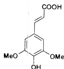
3,5-Dimethoxy-4-hydroxycinnamic acid
