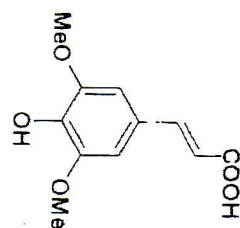
3,5-Dimethoxy-4-hydroxy cinnamic acid
